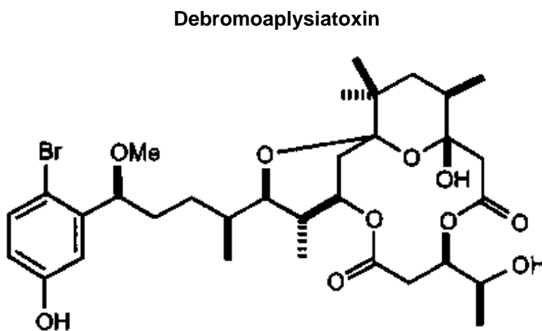
Figure 3.3 The chemical structures of debromoaplysiatoxin and lynghiatoxin-a
