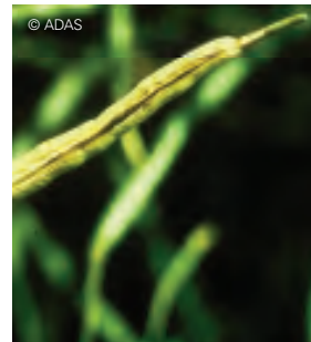
Brassica pod midge symptoms
