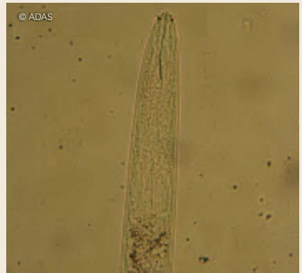
Stubby root nematode head region, showing curved spear used to penetrate plant roots
