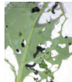
Turnip sawfly larvae and damage
