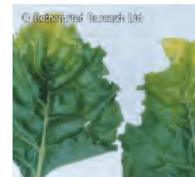
Capsid bug damage
