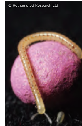
Spotted snake millipede
