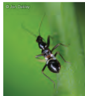
Damsel bug nymph ( Himacerus mirmicoides )
