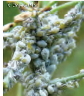
Mealy cabbage aphids on oilseed rape
