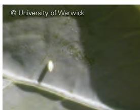
Small white butterfly egg
