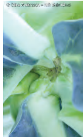
Damage due to swede midge larvae
