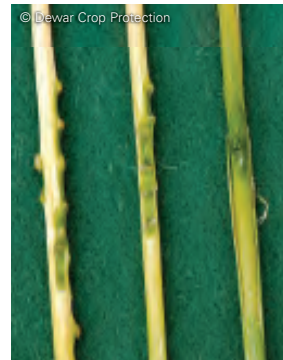
Saddle-shaped galls on wheat under the leaf sheath
