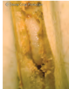
Rape winter stem weevil larva
