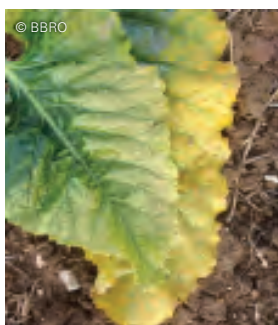
Symptoms of beet yellowing virus (top leaf) and beet mild yellowing virus (bottom leaf)
