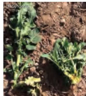
Rape winter stem weevil damage
