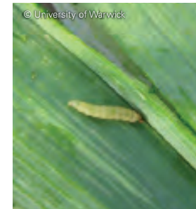
Leek moth larva
