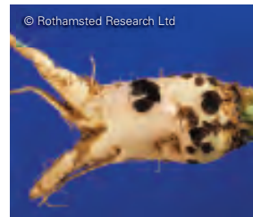
Cutworm damage to sugar beet
