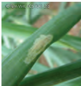
Allium leaf miner damage
