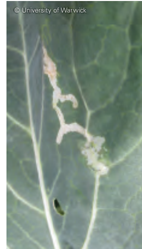
Brassica leaf miner damage
