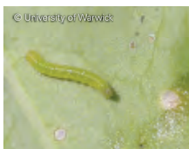
Small white butterfly larva
