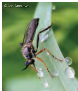
Robber fly (Dioctria rufipes)
