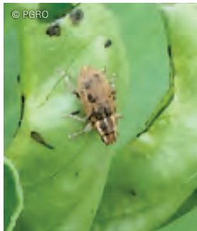
Pea and bean weevil
