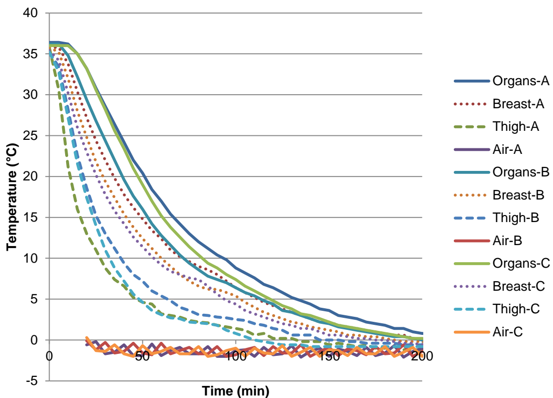
Figure 27. Chilling curves of three 1.5 kg partially-eviscerated broiler carcasses chilled trussed in air at -1.3 \pm 0.5^\circ\text{C} and 2.4 \text{ ms}^{-1}
