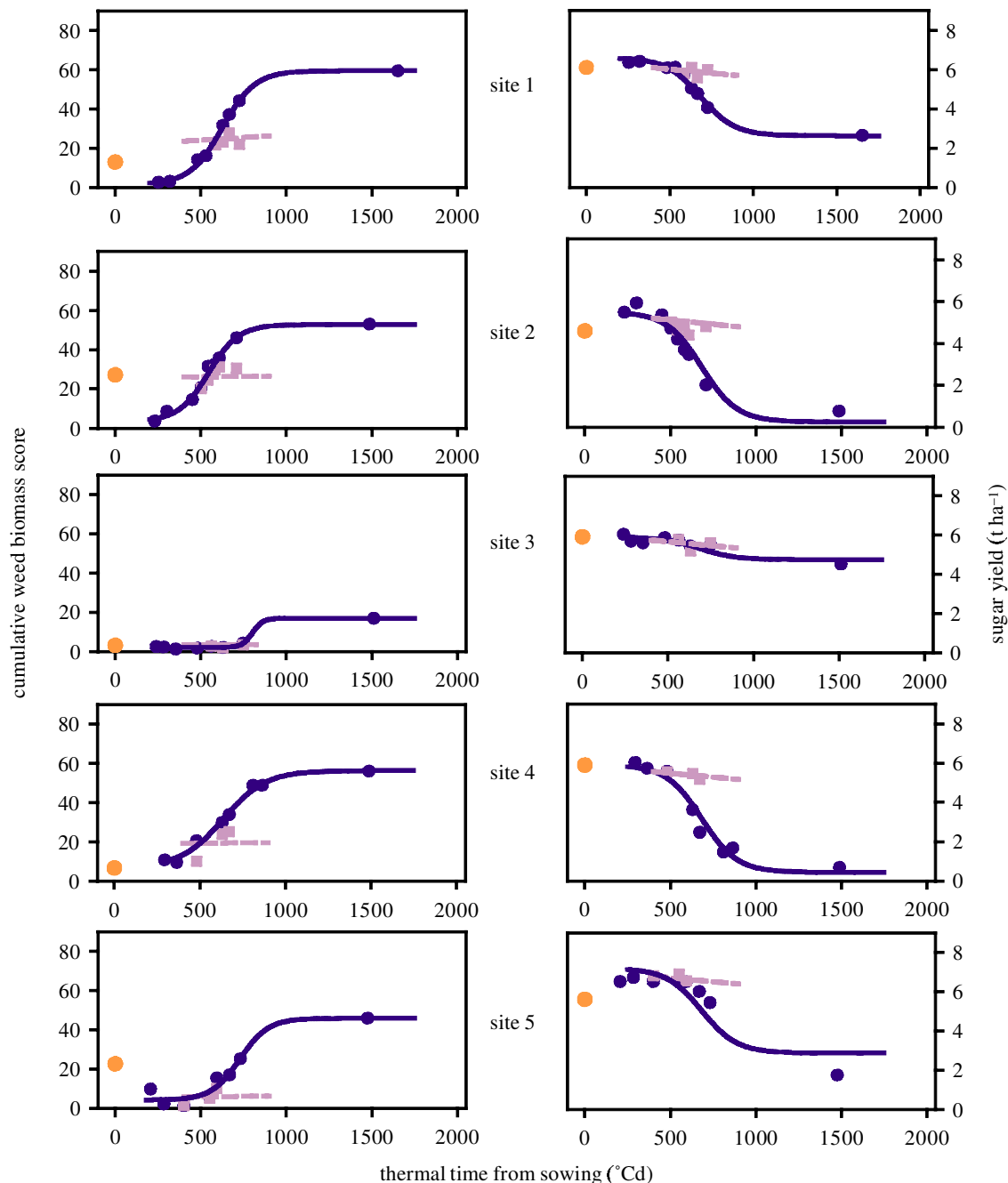
Figure 1. Effects of the timing ( ^{\circ}\text{Cd} after sowing) of the first overall sprays of glyphosate in a two spray regime (blue circles) and the second overall spray following a band spray (pink squares) on the cumulative biomass of weeds (left column figure) and sugar yield of sugar beet (right column figure) at five sites in 1999 and 2000. Data for conventional herbicides are given by orange circles.
