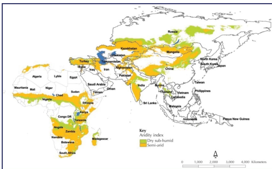
FIGURE 1 Projected tropical drylands of Africa and Asia in the year 2050, based on climate change models. The dryland tropics were delineated using the Aridity Index of the FAO and UNESCO (color figure available online).
