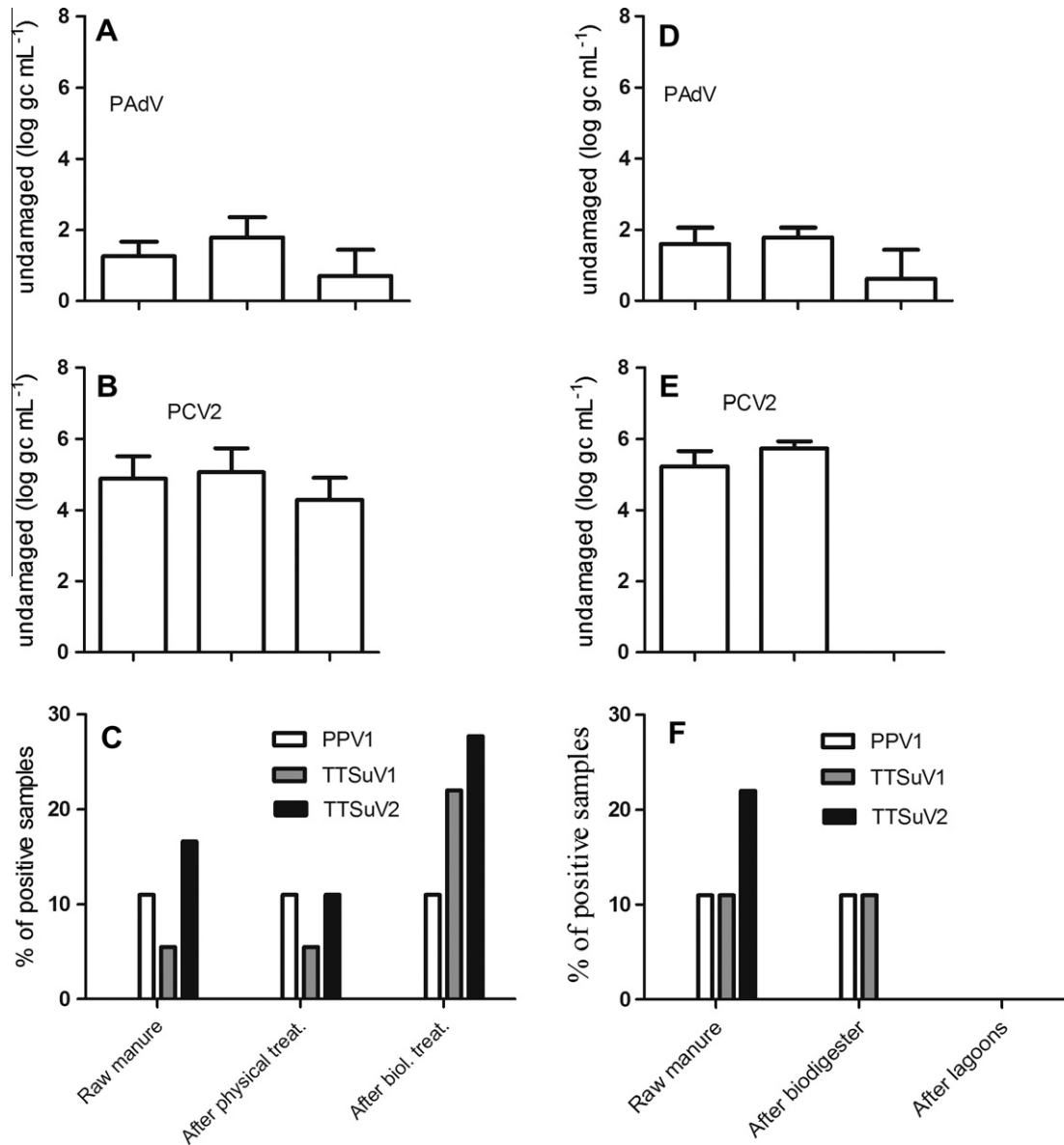
Fig. 3. Percentage of positive PPV1, TTV1 and TTV2 samples; average number of gc mL -1 of undamaged PAdV and PCV2 virus particles in System 1 (a–c) and in System 2 (d–f).
