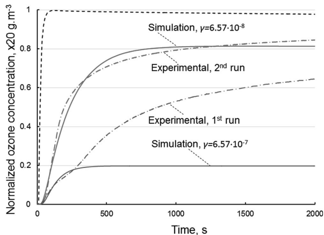
FIGURE 6. Simulated and experimentally obtained ozone concentration at the bottom of tube (18 mm wide and 90 mm deep) during ozone diffusion with reaction with tube walls (lettuce) taken into account. The dashed line shows ozone concentration inside the vessel.
