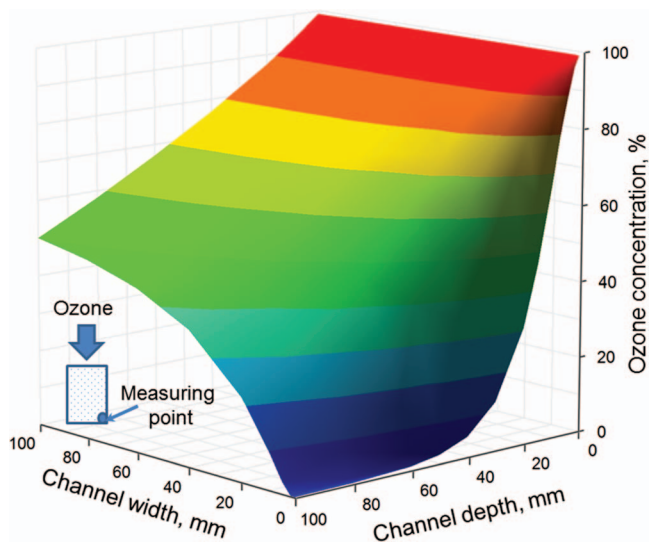
FIGURE 4. Simulated surface plot of the ozone equilibrium concentration in the bottom corner of a rectangular channel versus channel width and depth, calculated from the model.
