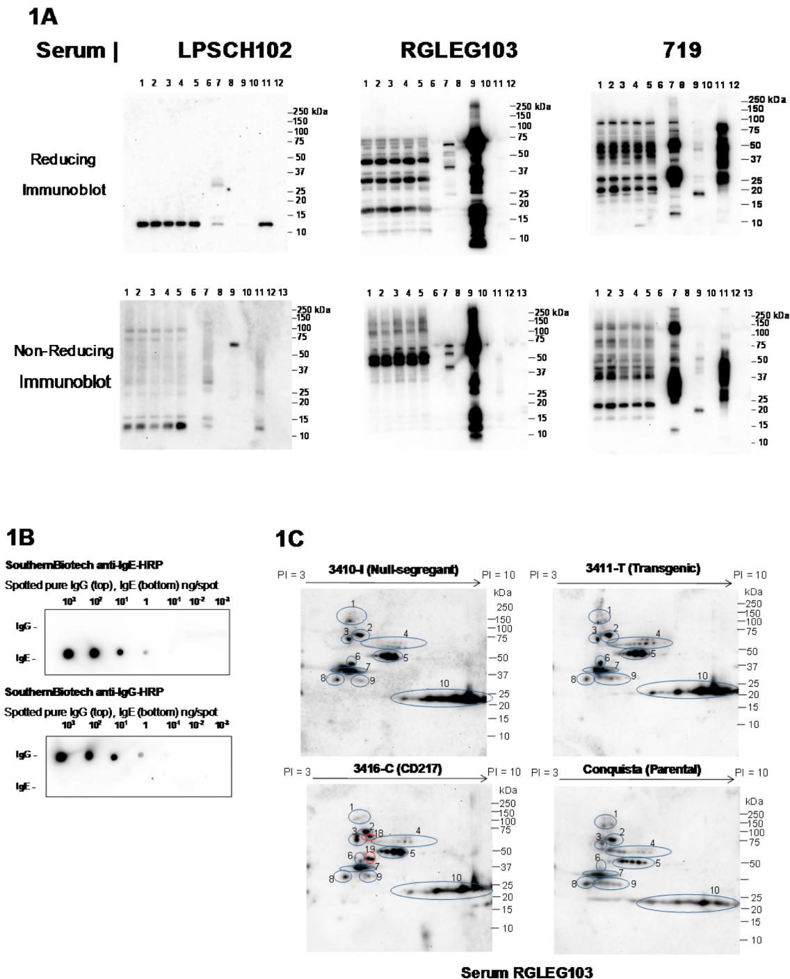
Figure 1. Soybean-allergic IgE binding to reduced and nonreduced proteins in 1D SDS-PAGE; BPS-CV127-9 (BASF). (A) Proteins in extracts of soybean (10 \mu\text{g} ), navy bean (10 \mu\text{g} ), peanut (2 \mu\text{g} ), and maize (10 \mu\text{g} ) were separated by SDS-PAGE under (a) reducing and (b) nonreducing conditions and immunoblotted with sera from three soybean-allergic subjects LPSCH102, RGLEG103, or 719 and detected using hIgE-specific mAb conjugated with HRP followed by ECL detection. Sample lanes: (1) 3410-I, null-segregant; (2) 3411-T, GM line BPS-CV127-9; (3) 3415-M, MON8001; (4) 3416-C, CD217; (5) Conquista, parental line; (6) none; (7) navy bean; (8) none; (9) peanut; (10) none; (11) maize; (12) MW marker. (B) Samples of purified human IgE and IgG were diluted and spotted onto nitrocellulose, representing from 1 pg–1 \mu\text{g} of immunoglobulin and then detected using monoclonal anti-hIgE or anti-hIgG to demonstrate immunoglobulin specificity. (C) Protein samples of null-segregant 3410-I GM, 3411-T, CD217, 3416-C, and Conquista (parental) soybean lines were separated by IEF in pI 3–10 nonlinear IPG strips then by size in SDS-PAGE, blot incubated, with serum RGLEG103.
