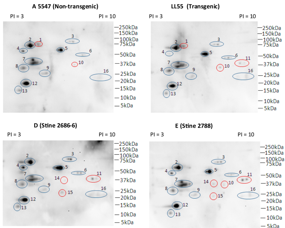
Figure 4. Serum IgE immunoblots to Bayer LL55 soybeans with soybean allergic plasma 20197-BH using 1D SDS-PAGE samples under reducing and nonreducing conditions and 2D PAGE. Sample lanes (1D blots): (1) A5547 (near-isogenic); (2) LL55 (transgenic); (3) Stine 2686-6; (4) Stine 2788; (5) Stine 3000-0; (6) empty; (7) MW marker; (8) empty; (9) navy bean; (10) empty; (11) peanut; (12) empty; (13) maize (corn). No obvious difference in binding between soybean samples was visible from 1D blots beyond the more intense band at 250 kDa in the three commercial lines (lanes 3–5). A few low-intensity spots differed in 2D PAGE blots. Two spots that were visible in LL55 transgenic in circle 11 were not visible in the A5547 nontransgenic line but were also visible in both D and E samples. In addition, the faint spots in circles 14 and 15 were visible in D and E, but not the LL55 transgenic or nontransgenic A5547.
