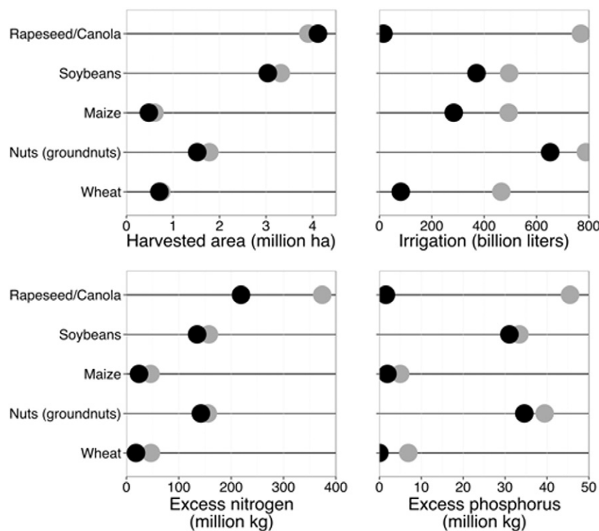
Fig. 3. Estimated resource use associated with the estimated harvested area for the top five aquaculture feed crops circa 2008. The grey points represent the 'global' production scenario. The black points represent the 'exporting country' scenario, where production is assumed to take place in the top three exporting countries. Comparison among the five crops in terms of potential cropland harvested area (hectares), irrigation water consumption (liters), excess nitrogen (N), and excess phosphorus (P) are shown.
