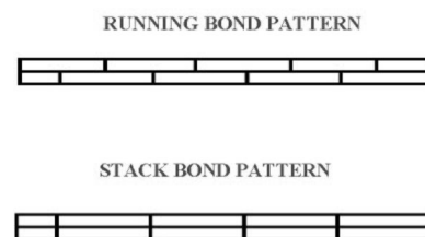
Figure 1. Bond Patterns on Concrete Block Walls
