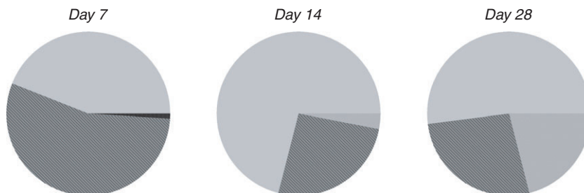
Figure 6 Pie charts showing the relative abundance of bacterial class in the three clone libraries from days 7, 14 and 28 at steady-state conditions.
