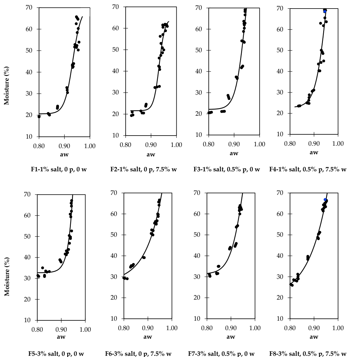
Figure 2. Relation between the water activity (aw) and moisture in cured sausages with different formulations. p—phosphate; w—wine.
