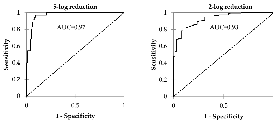
Figure 6. Receiver operating characteristic curves (ROC) of logistic regression models to predict the Salmonella population's 5- and 2-log reduction.
